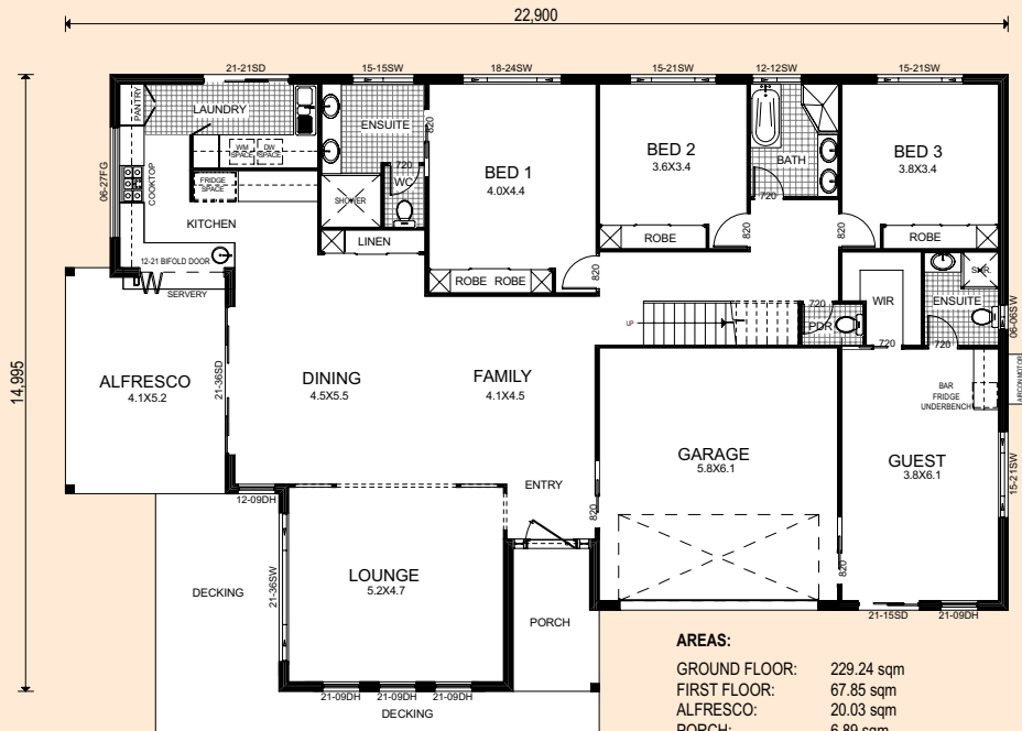
GROUND FLOOR LAYOUT
